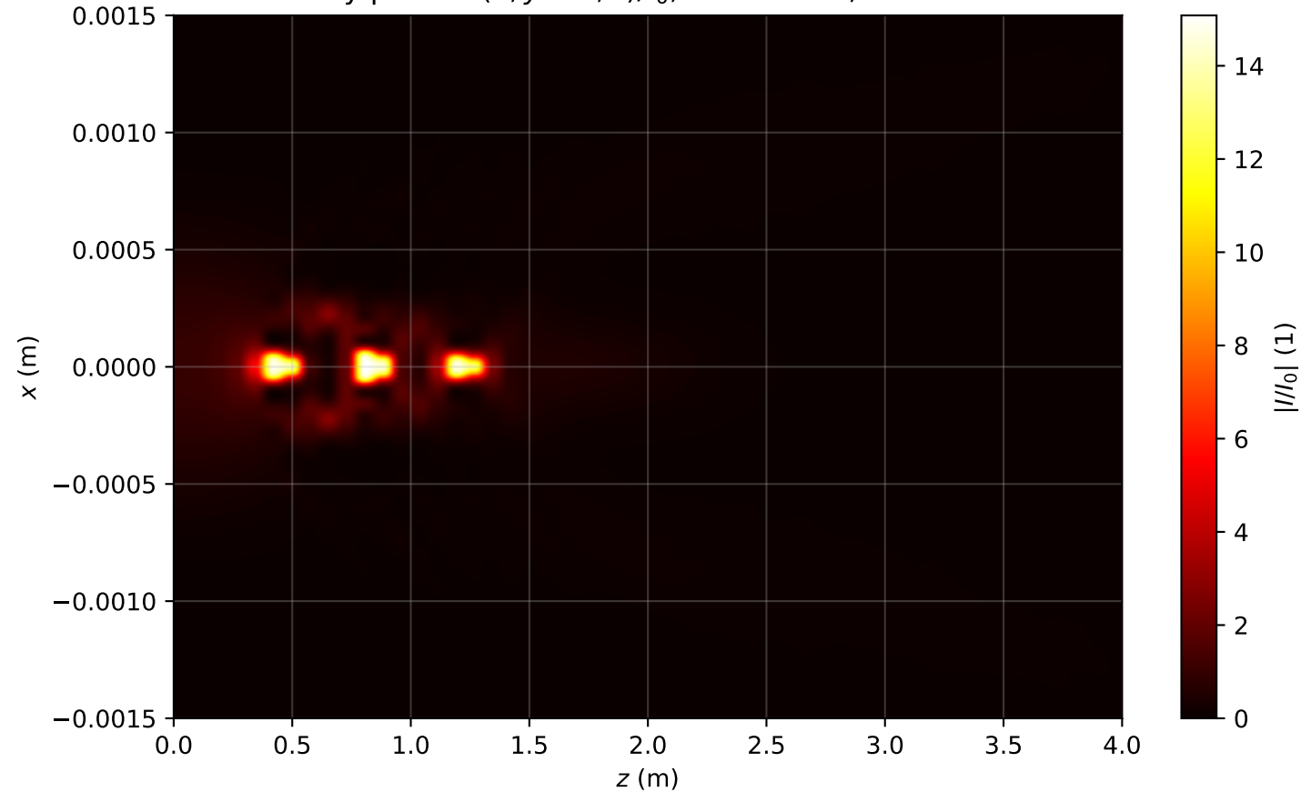
Intensity profile I(x, y = 0, z)/I_0 , P_{in}=7.5P_{cr} , artificial time
